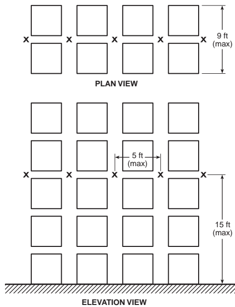
FIGURE 16.6.4(c) Double-Row Rack Sprinkler Layout 8 — Option #2.
