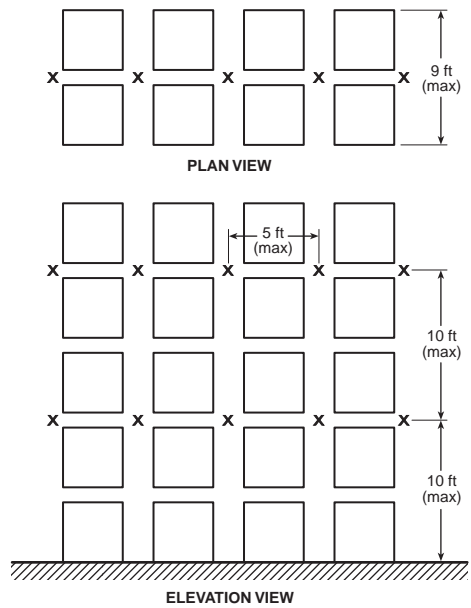
FIGURE 16.6.4(e) Double-Row Rack Sprinkler Layout 9 — Option #2.
