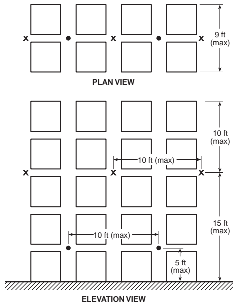
FIGURE 16.6.4(b) Double-Row Rack Sprinkler Layout 8 — Option #1.
